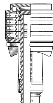
D4TL D4TL NOZZLE + TA ADAPTOR
