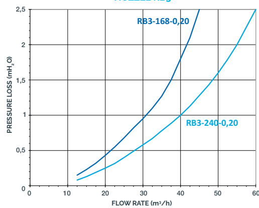
NOZZLE RB3
